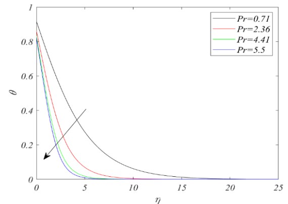
Fig. 12. Variations of Pr on temperature
